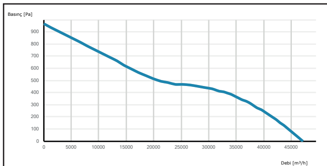
TAXI 900-8-40
