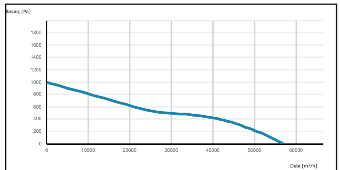
BAXI 1000-8-40
