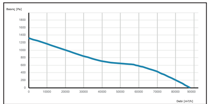
CTAXI 1120-8-40
