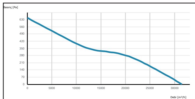
CAXI 800-5-35
