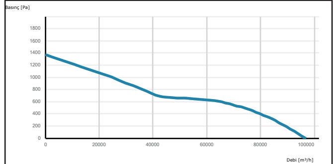
HAXI 1120-8-45
