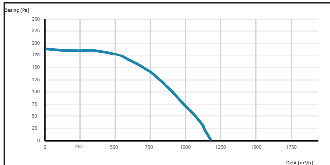
HMEF 280
