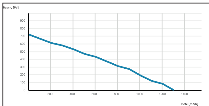
SHU 13
