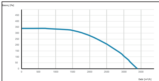
CRAD 400
