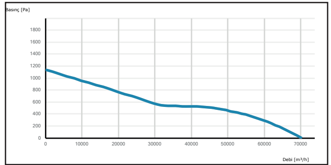
CAXI 1000-8-45
