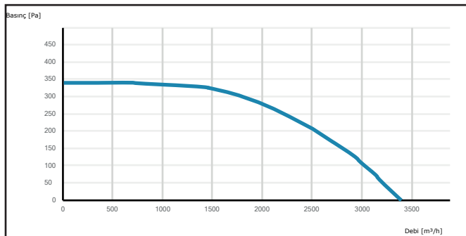
REC 60-35
