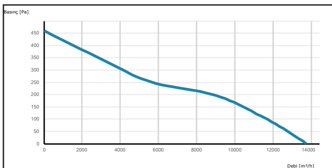
CAXI 630-5-30
