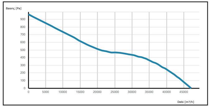
CAXI 900-8-40
