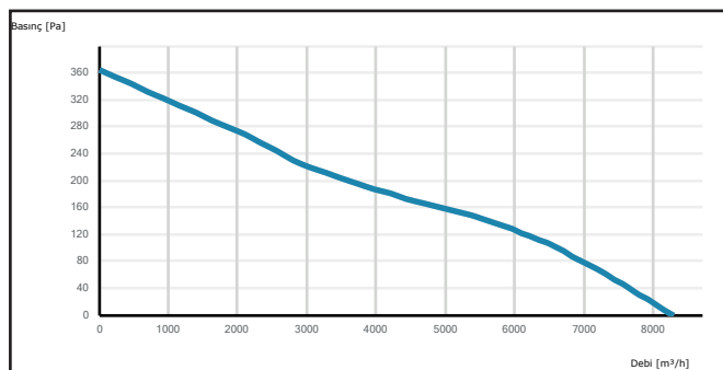
CAXI 560-5-25
