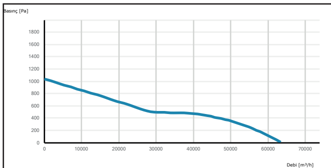
BAXI 1000-8-45
