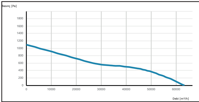
CAXI 1000-8-40
