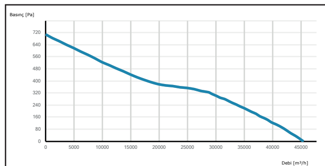
CAXI 900-5-40
