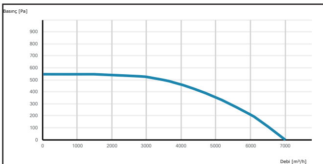
CRAD 500
