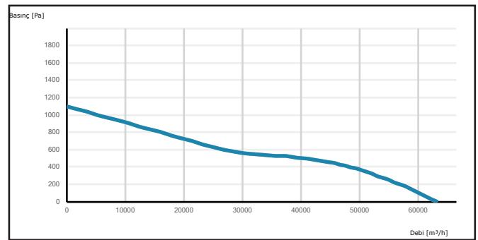
CTAXI 1000-8-40
