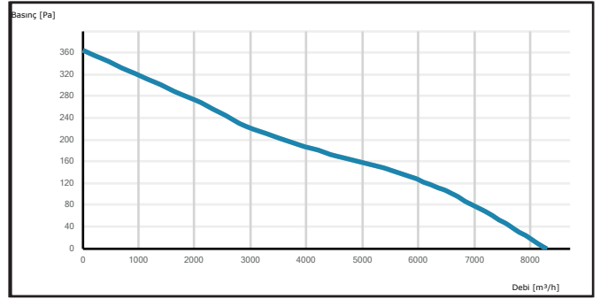
HAXI 560-5-25
