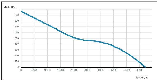
CTAXI 900-8-40
