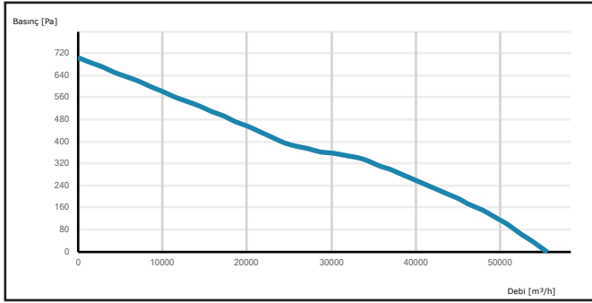
AXI 1000-5-40
