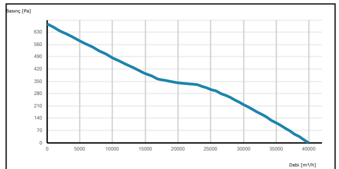
TAXI 900-5-35
