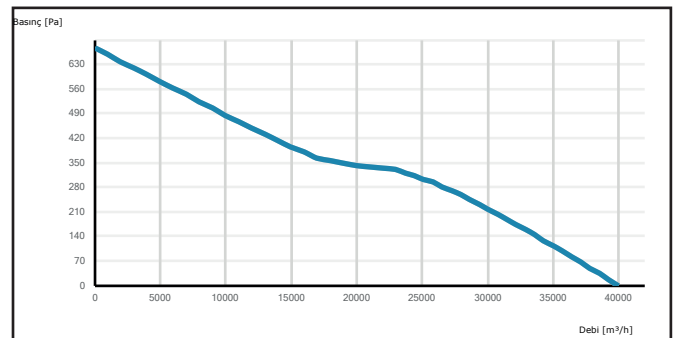
TAXI 900-5-35
