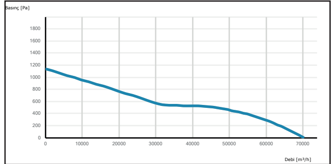
HAXI 1000-8-45
