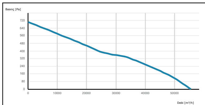
PAXI 1000-5-40
