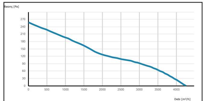
CAXI 450-5-25
