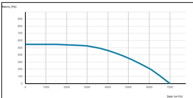
REC 80-50
