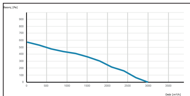
SHU 30
