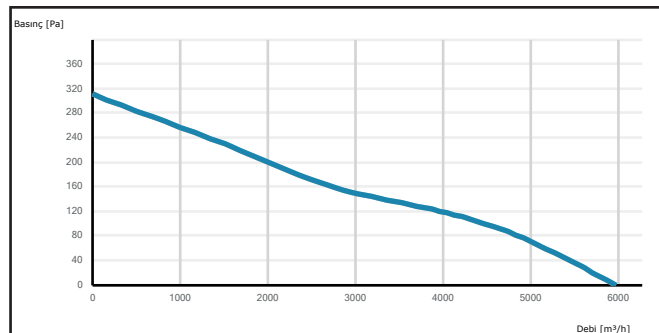
TAXI 500-5-25
